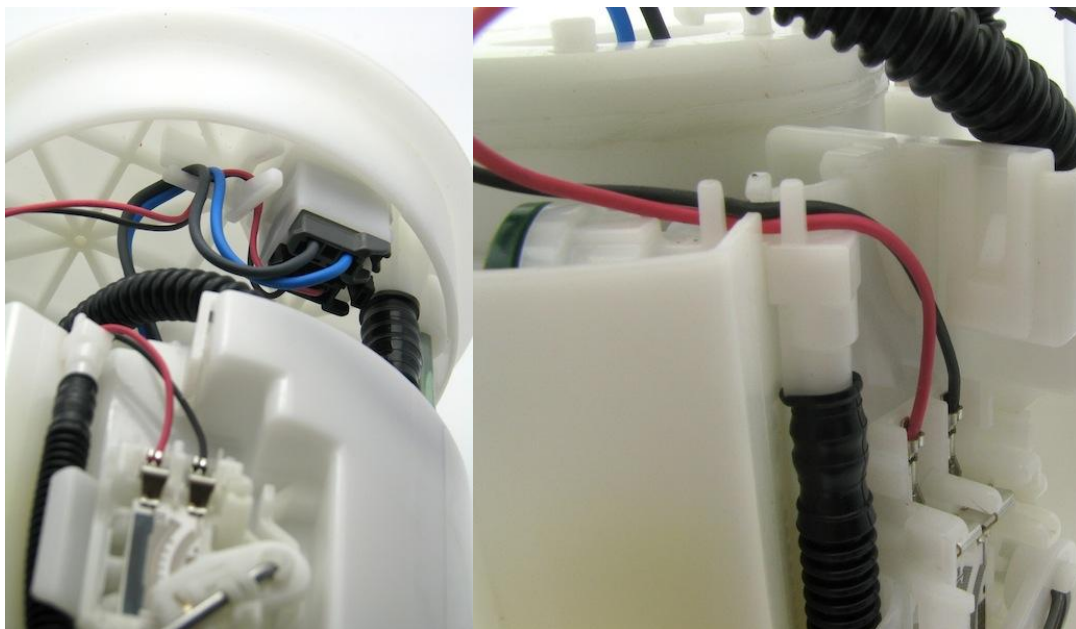
Routing of the wires for reference.
